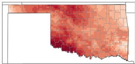
Map 1: Number of Days Over 95°F, Average from 1981-2005
