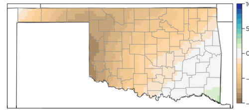
Map 2: Percentage Change in Total Annual Precipitation, Moderate Climate Scenario, Average from 2035-2065
