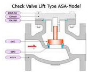
Lift Check Valve
