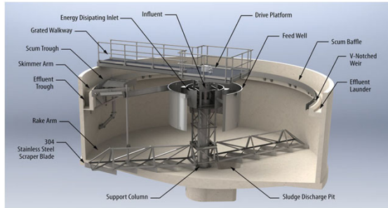
Cross section of circular clarifier
