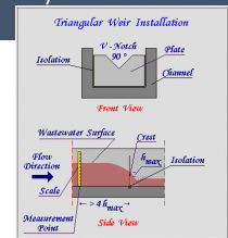
Staff gauge
