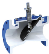
Swing Check Valve
