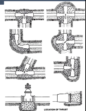
LOCATION OF THRUST
